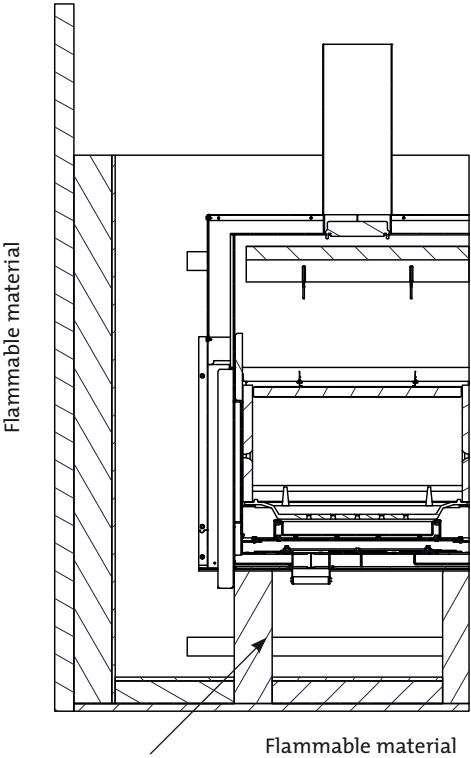
Supporting of stove on non-flammable side pieces
